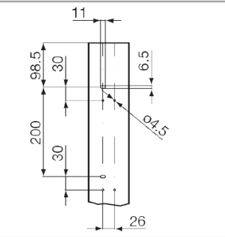
TerCia TA-C45 90x55 Perforation socle
