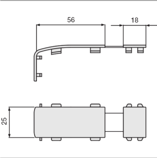
GAS - Joint de socle Dimensions
