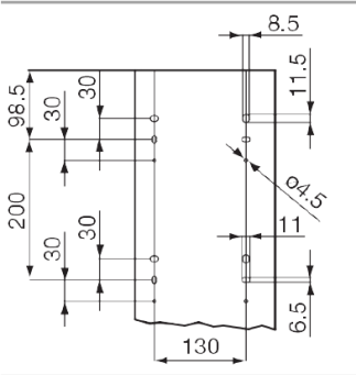
TerCia TA-C45 200x55 Perforation socle
