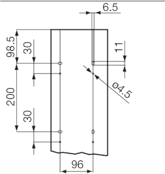
TerCia TA-C45 164/3x55 Perforation socle
