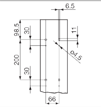
TerCia TA-C45 134/2x55 et 164/2x55 Perforation socle
