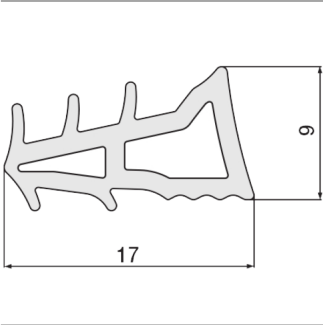
JDS-C - Joint de sol souple Dimensions
