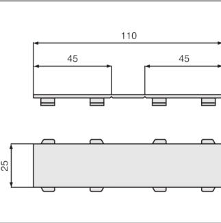
GAC - Joint de couvercle Dimensions
