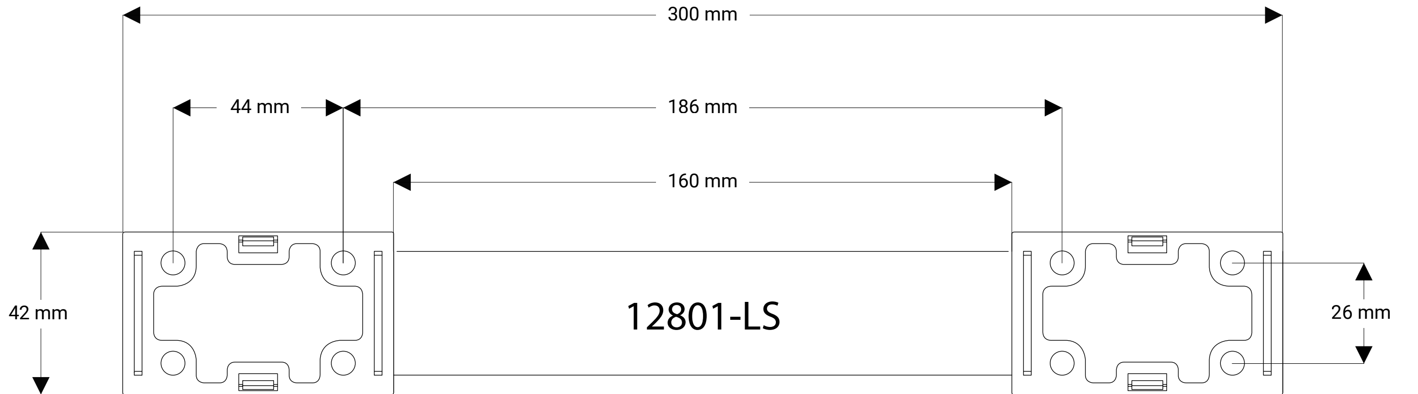
300mm Grab Rail Assembly (Fitting Template)
