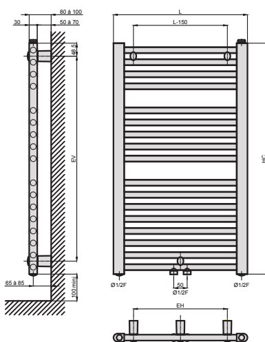
VERSION EAU CHAUDE RACCORDEMENT CENTRAL 50 MM
