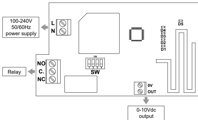
Fig. 1: Electronic board
