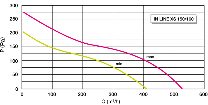
Courbe aéraulique XS 150
