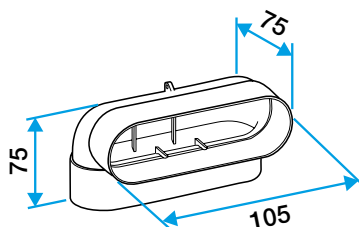
Coude vertical 90°
