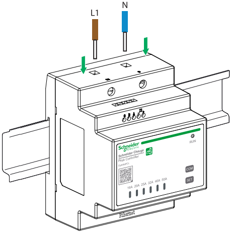
220-240V AC 1-Phase
