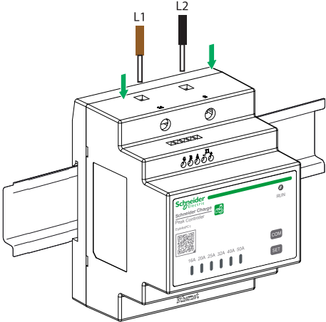
220-240V AC 1-Phase No Neutral
